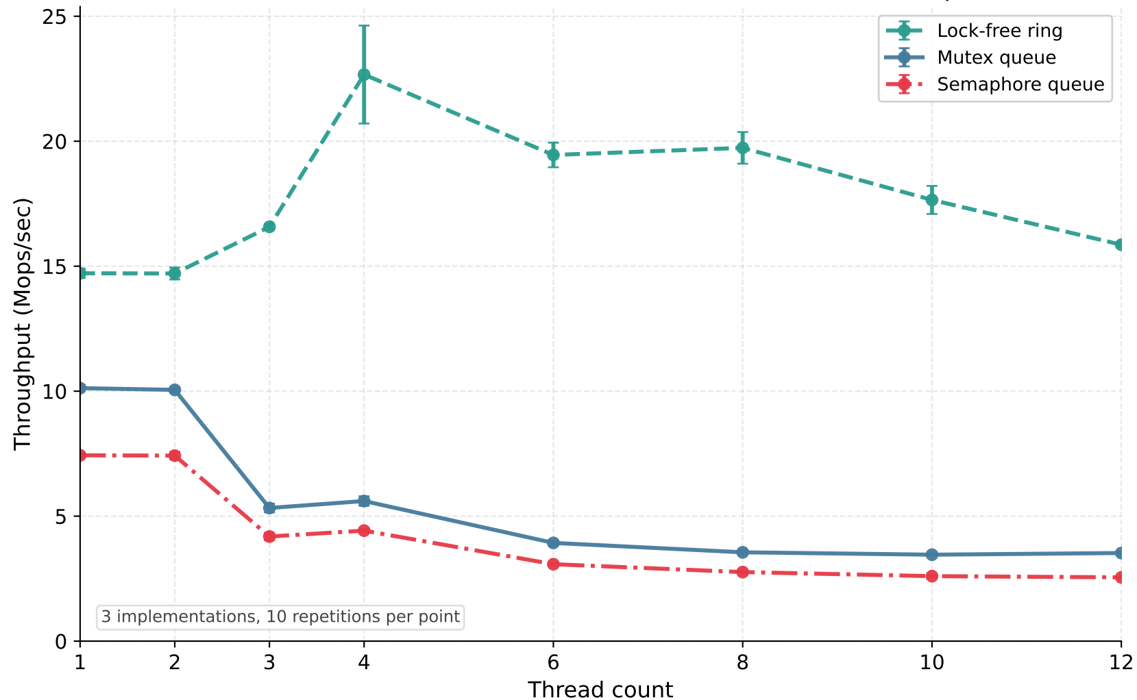
Bounded Producer-Consumer Queue - Small-buffer hotspot
